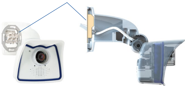
Space for RJ45 wall outlet/concealed cabling
